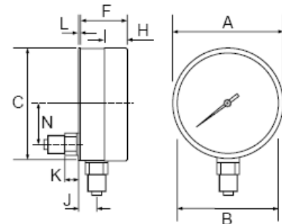
501T Vertical Entry, Direct Mounted
